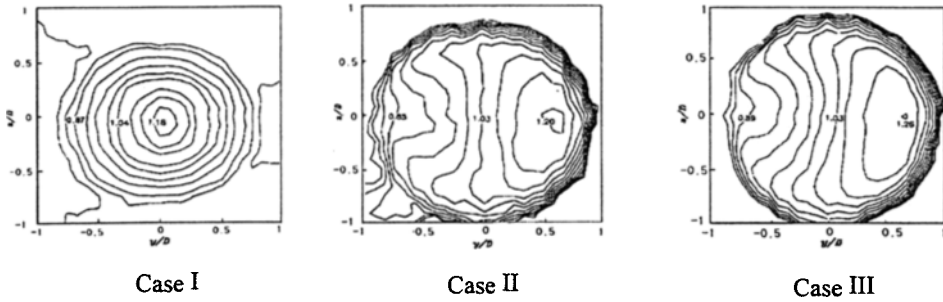
Fig. 4 Constant velocity contours at the jet exit for Case I, II, III
