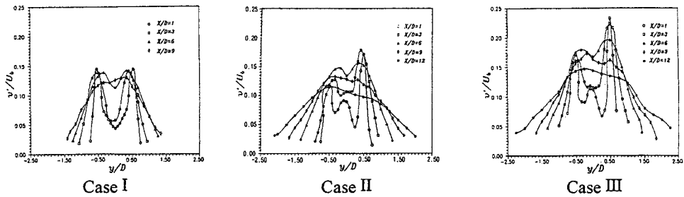
Fig. 8 v' profiles for Case I, II, III
