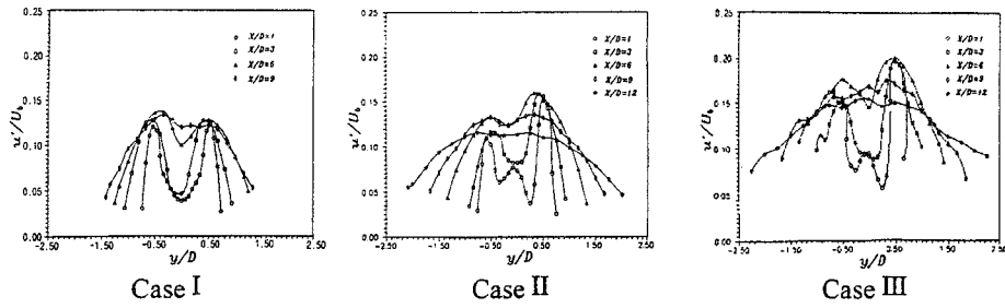
Fig. 7 u' profiles for Case I, II, III
