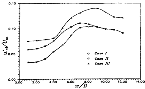
Fig. 9 Axial distribution of u' along the center-line of jet
