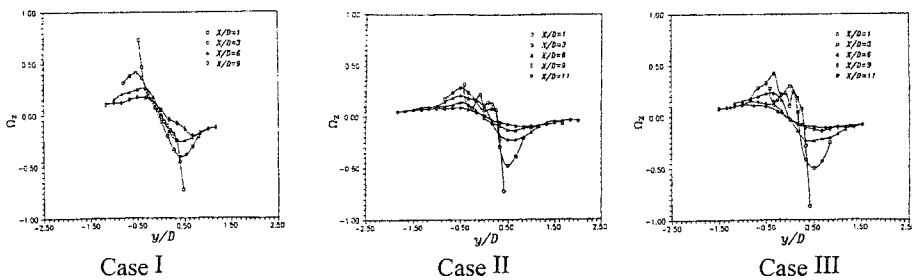
Fig. 12 Vorticity profiles for Case I, II, III
